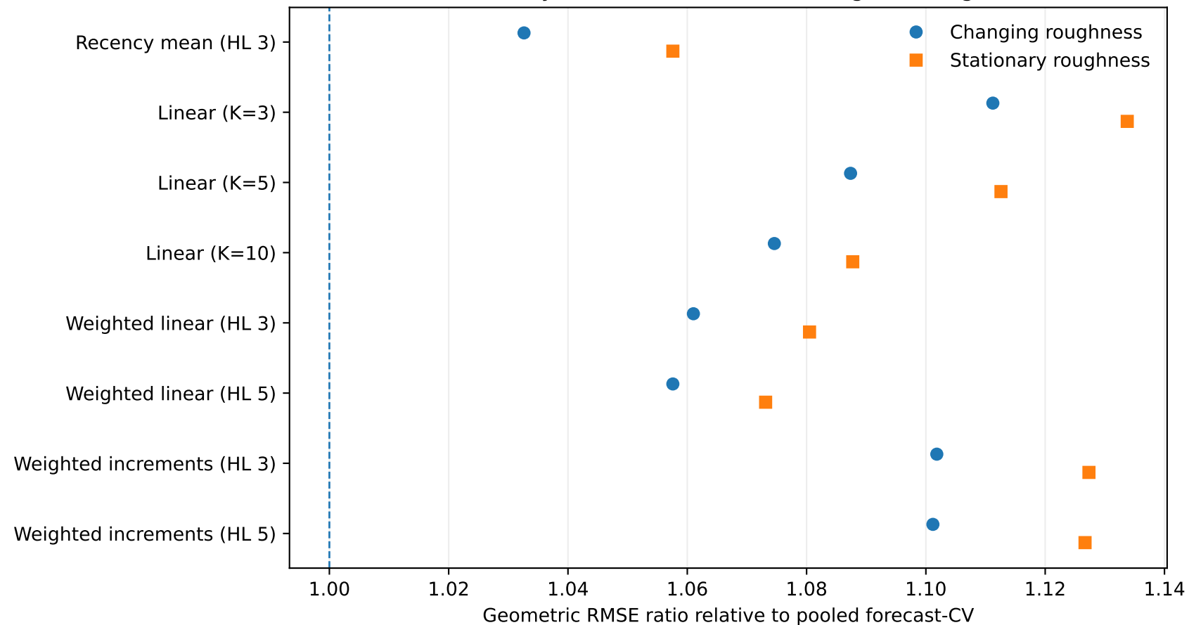
Rule-family behavior under latent roughness regimes
